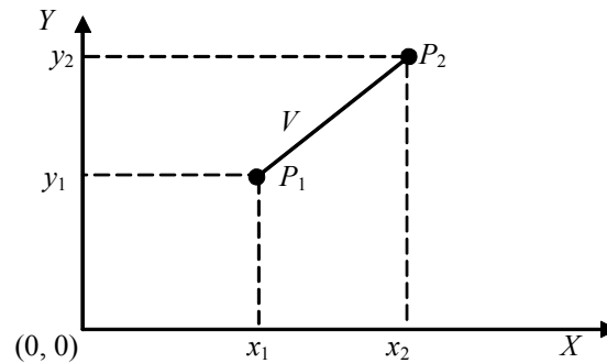
Fig. 2.7 Vector Representation
