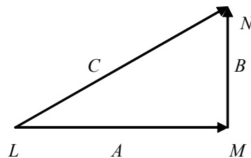
Fig. 2.10 Addition of Two Vectors
