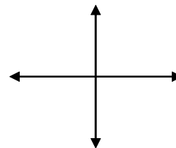
Fig. 3.8 Four-Connected Approach
