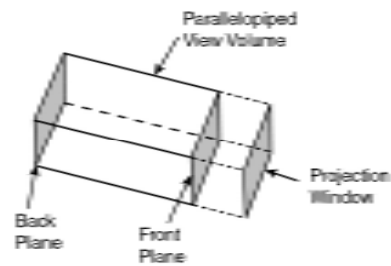
Fig. 11.3 Parallel projection
