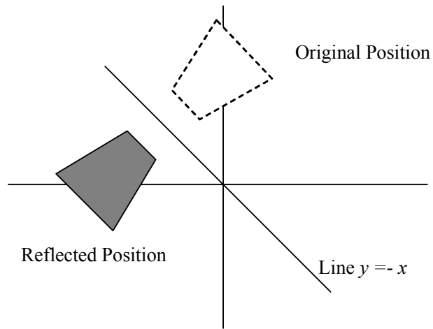
Fig. 4.11 Reflection with Respect to the Line y = -x
