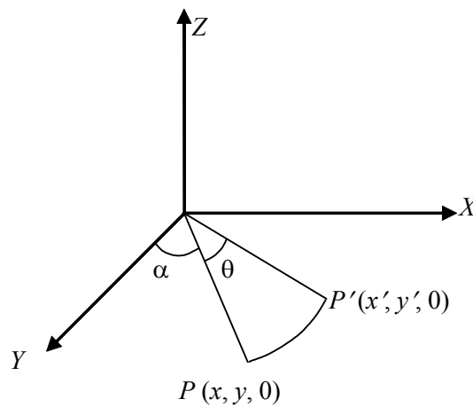
Fig. 10.6 Rotation about z-axis
